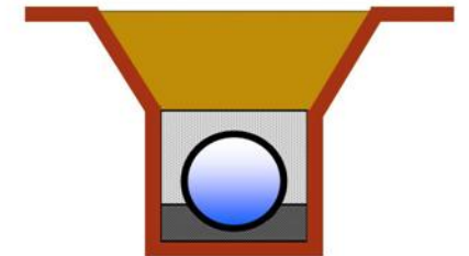
FLEXIBLE PIPE INSTALLATION
