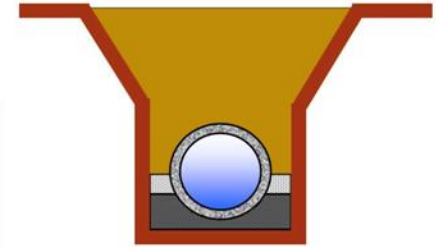
RCP TYPE 1 INSTALLATION
