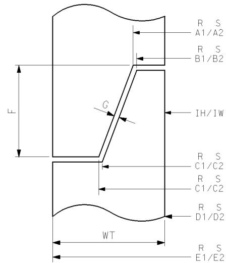
JOINT DETAIL
