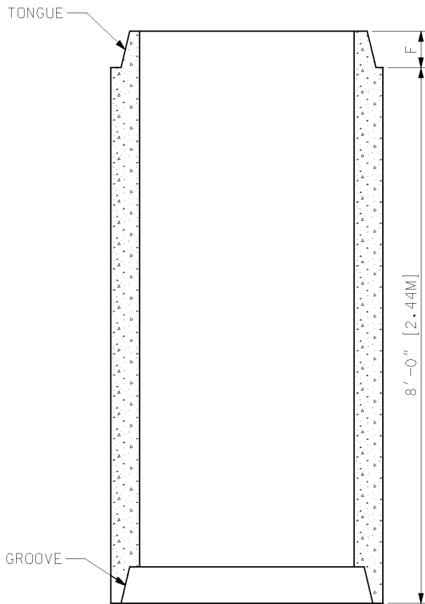
REINFORCED CONCRETE ELLIPTICAL PIPE
