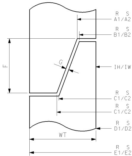
JOINT DETAIL
